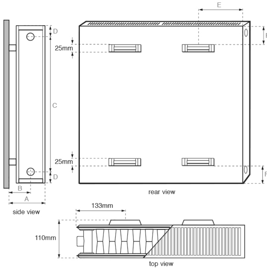
MILANO DEEP HORIZONTAL PLAN DIMENSIONS (mm)
